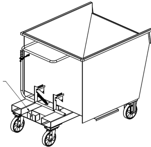
VASCHETTA PORTA CATENA CHAIN STORAGE COMPARTMENT
